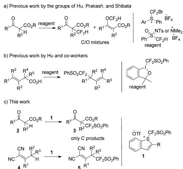
Scheme 1. Difluoromethylation and (phenylsulfonyl)difluoromethylation of \text{C}_{\text{sp}^3} -centered nucleophiles. Tf = trifluoromethanesulfonyl.
